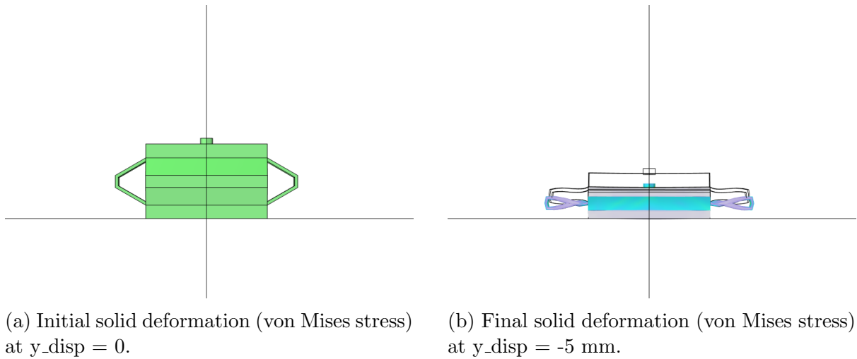
Figure 13: Solid mechanics simulation showing stress distribution at initial and final displacement.
