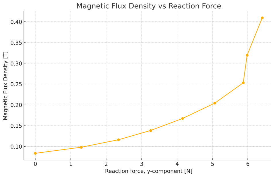
Figure 24: Applied force vs Magnetic flux density change
