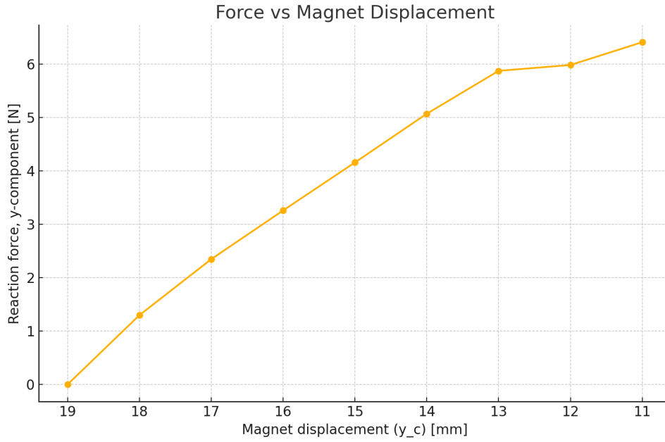
Figure 23: Force experienced by sensor with respect to the displacement of the magnet
