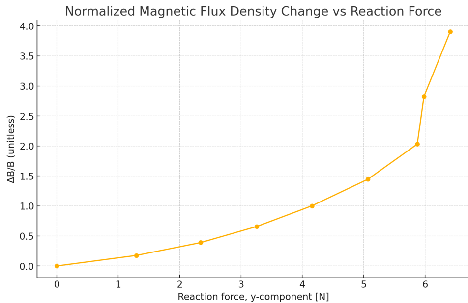
Figure 26: Normalized Magnetic Flux Density Change vs Reaction Force
