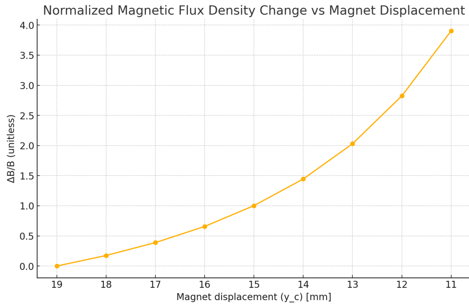
Figure 25: Normalized Magnetic Flux Density Change vs Magnet Displacement
